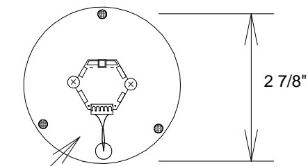
Heat Sink 10 Watt LED
